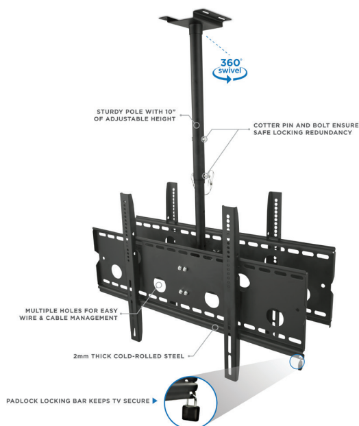
VESA COMPLIANT ARM BRACKETS FITS VESA PATTERNS UP TO 800 mm X 450 mm
