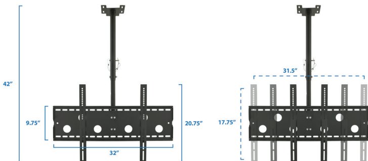
VESA COMPLIANT ARM BRACKETS FITS VESA PATTERNS UP TO 800 mm X 450 mm
