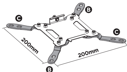
VESA 200x200
