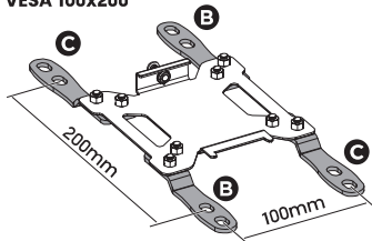
VESA 100x200
