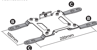
VESA 200x100
