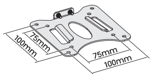
VESA 75x75 100x100
