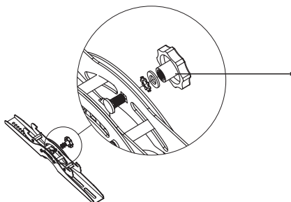
(2)Plastic Knob
