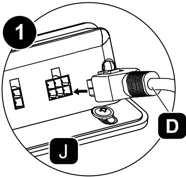
Motor to control panel
