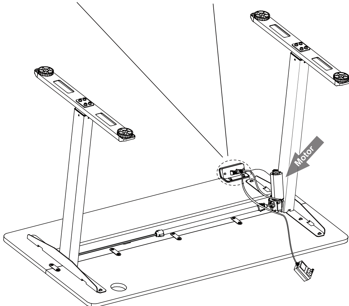
Motor to control panel
