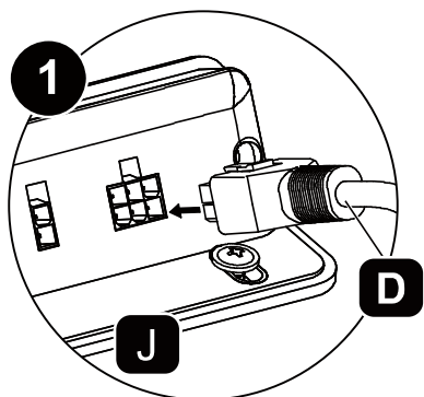
Motor to control panel
